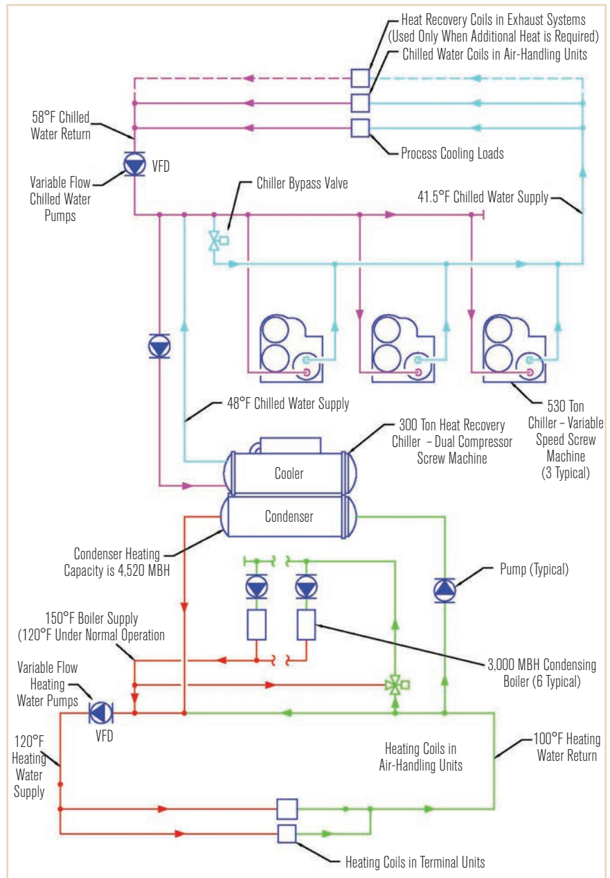
FIGURE 3: Heat recovery system.
