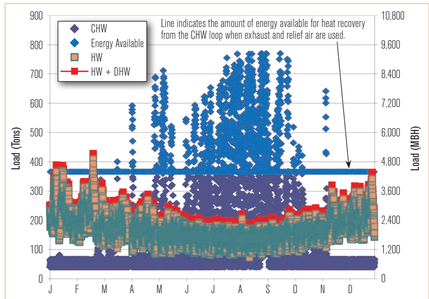
FIGURE 2: Building hydronic hourly loads.
